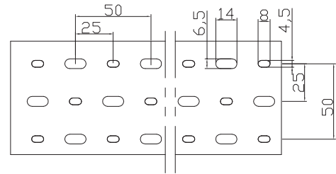
样式: 75mm~140mm宽
