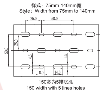
样式: 75mm-140mm宽
