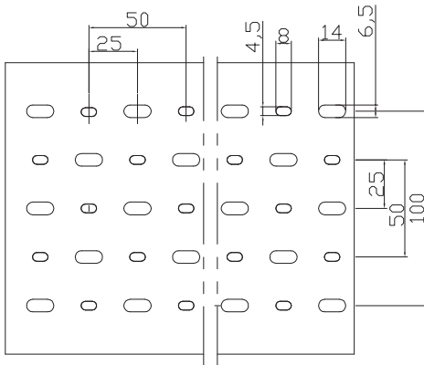
样式: 150mm~200mm宽
